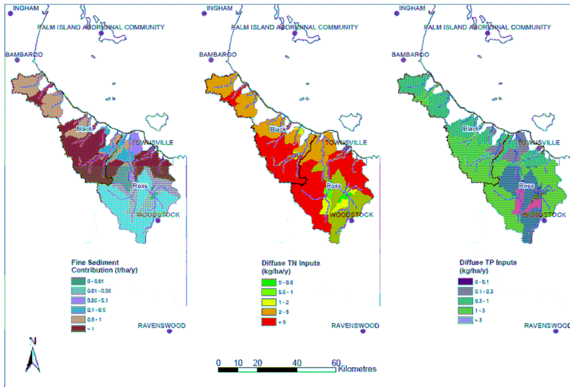
Figure 3-1 Estimated pollutant contributions Black and Ross River Basins
