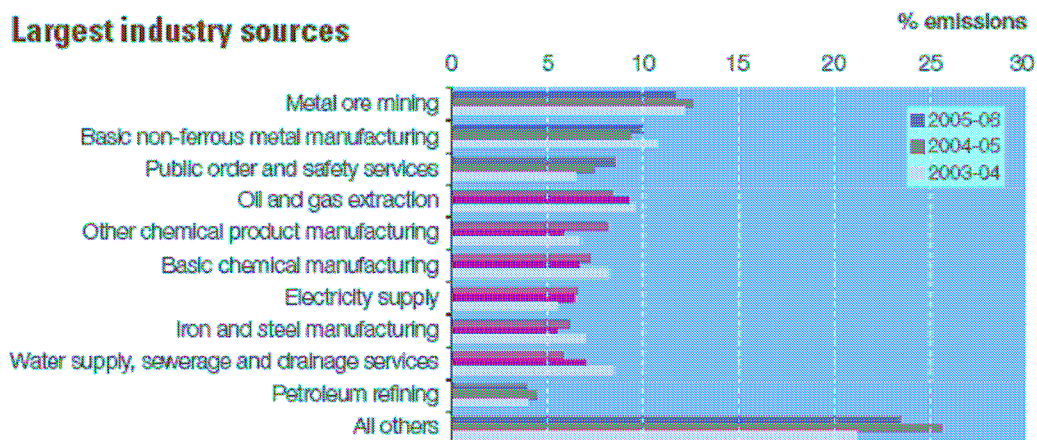
Figure 2-3 Main Industry Emission Sources
