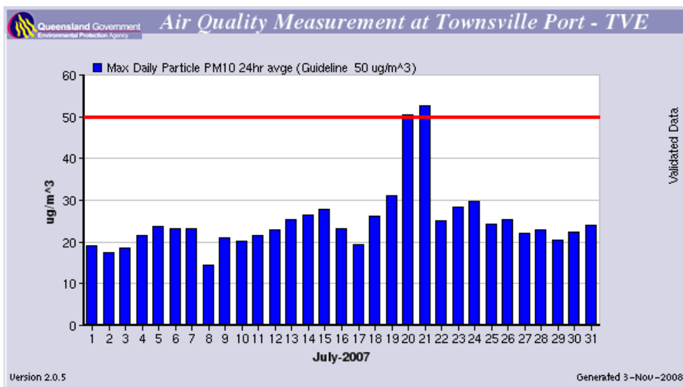
Figure 4-4 Townsville Port Air Quality by Month (July 2007)
