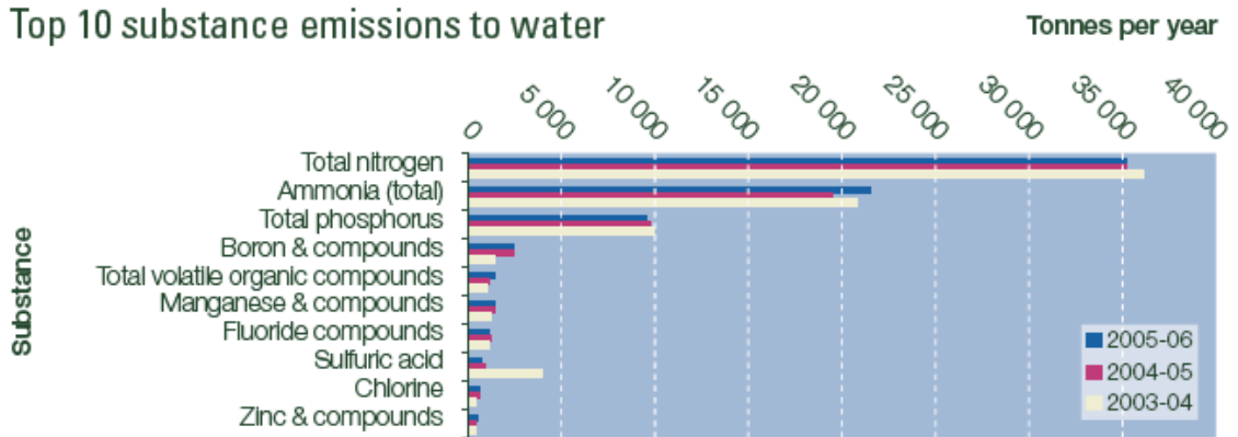
Figure 2-4 Australian Top Ten Emission Substances to Water
