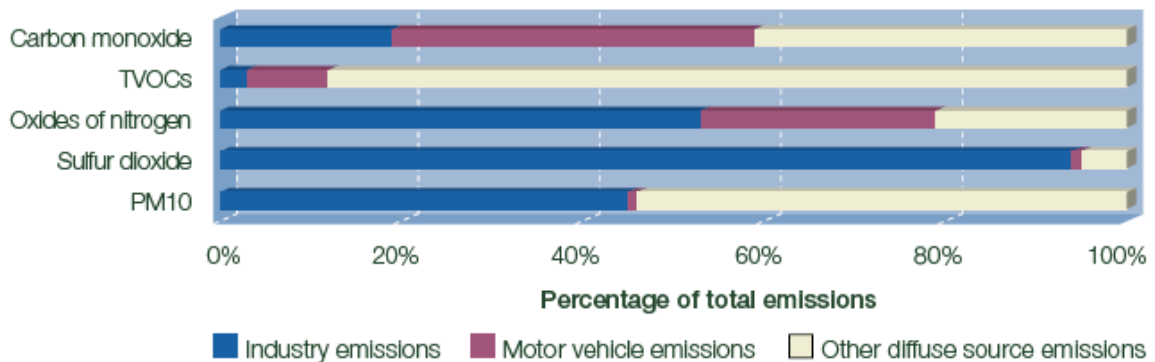
Figure 2-6 NPI Top Five Substances Emitted to Air in Australia 2005-06
