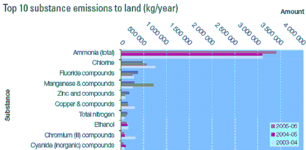
Figure 2-5 Australian Top Ten Land Emissions
